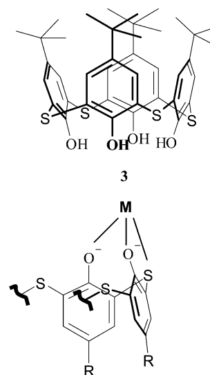
Fig. 1. Coordinated Zn(II) with 5,11,17,23-tetra- tert -butyl-2,8,14,20-tetrathiacalix[4]arene (compound 3 ). For clarity, partly drawing of 3 . General assumption of coordinated metals with thiocalix[4]arene in [10].
