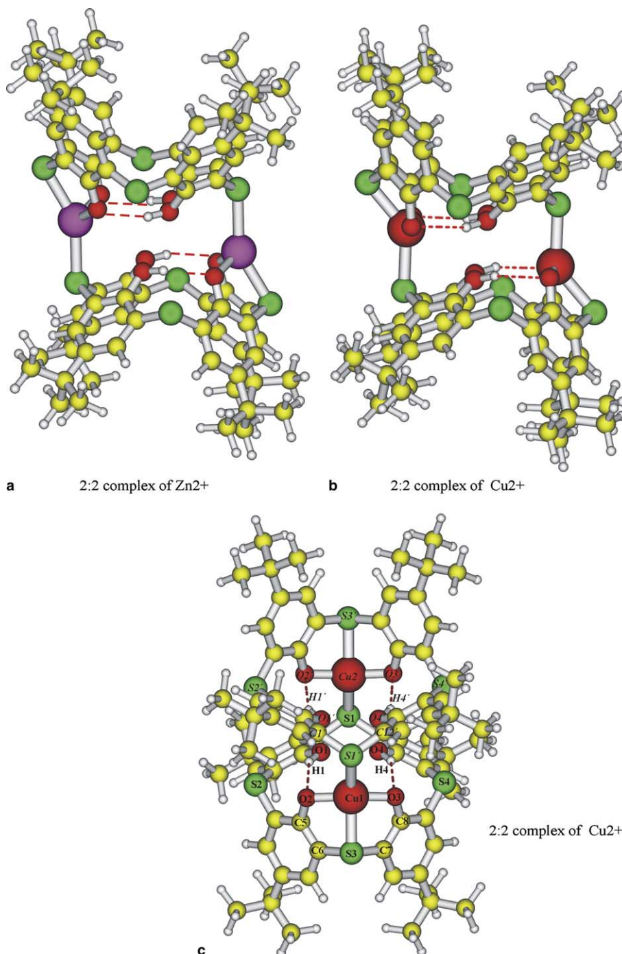
Fig. 6. Optimized structures of each 2:2 metal complex of 3 obtained at AM1 method.
